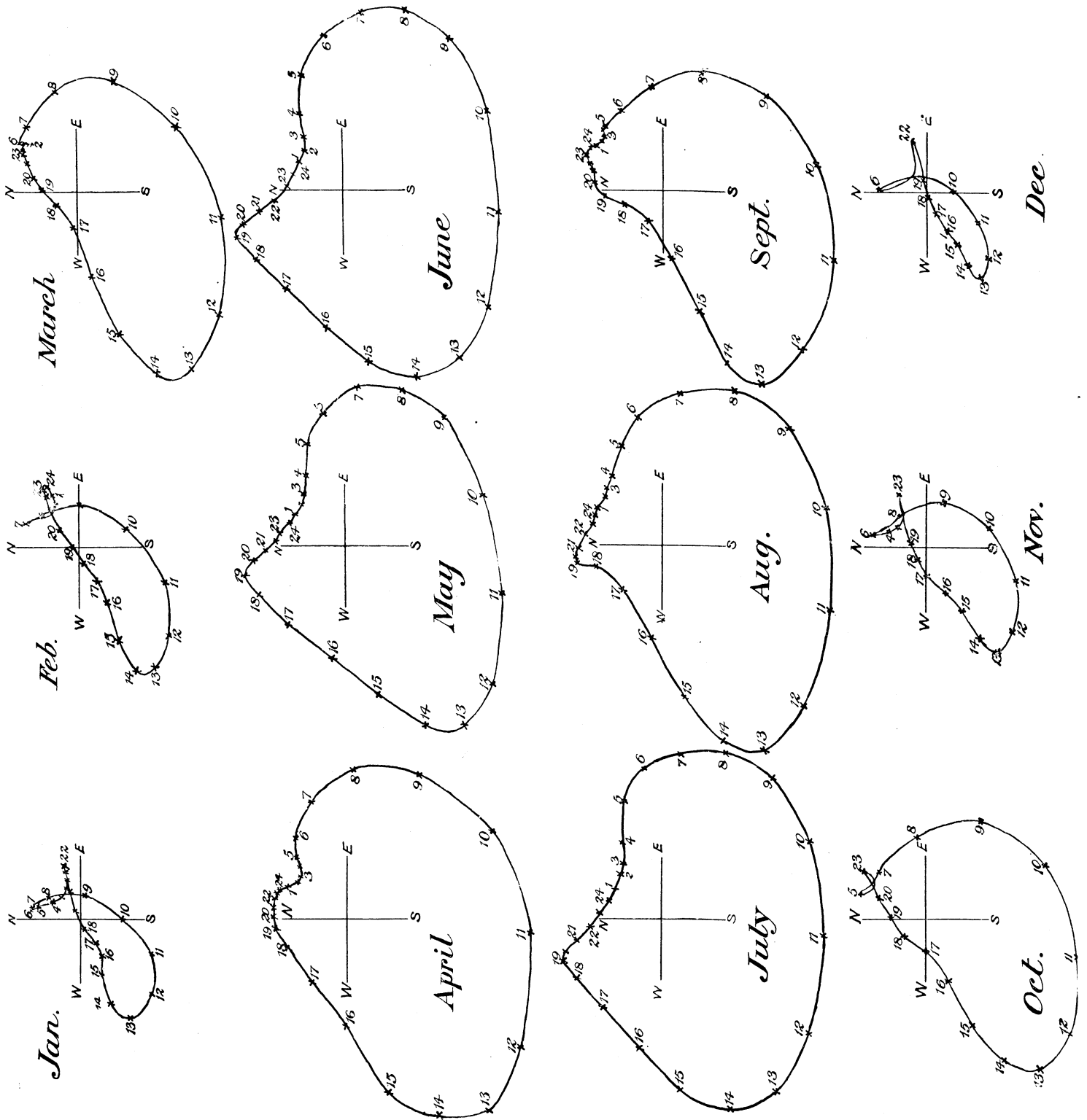
Fig. 8. Vector diagrams in horizontal plane (11 years). Arms of cross each 10γ.
