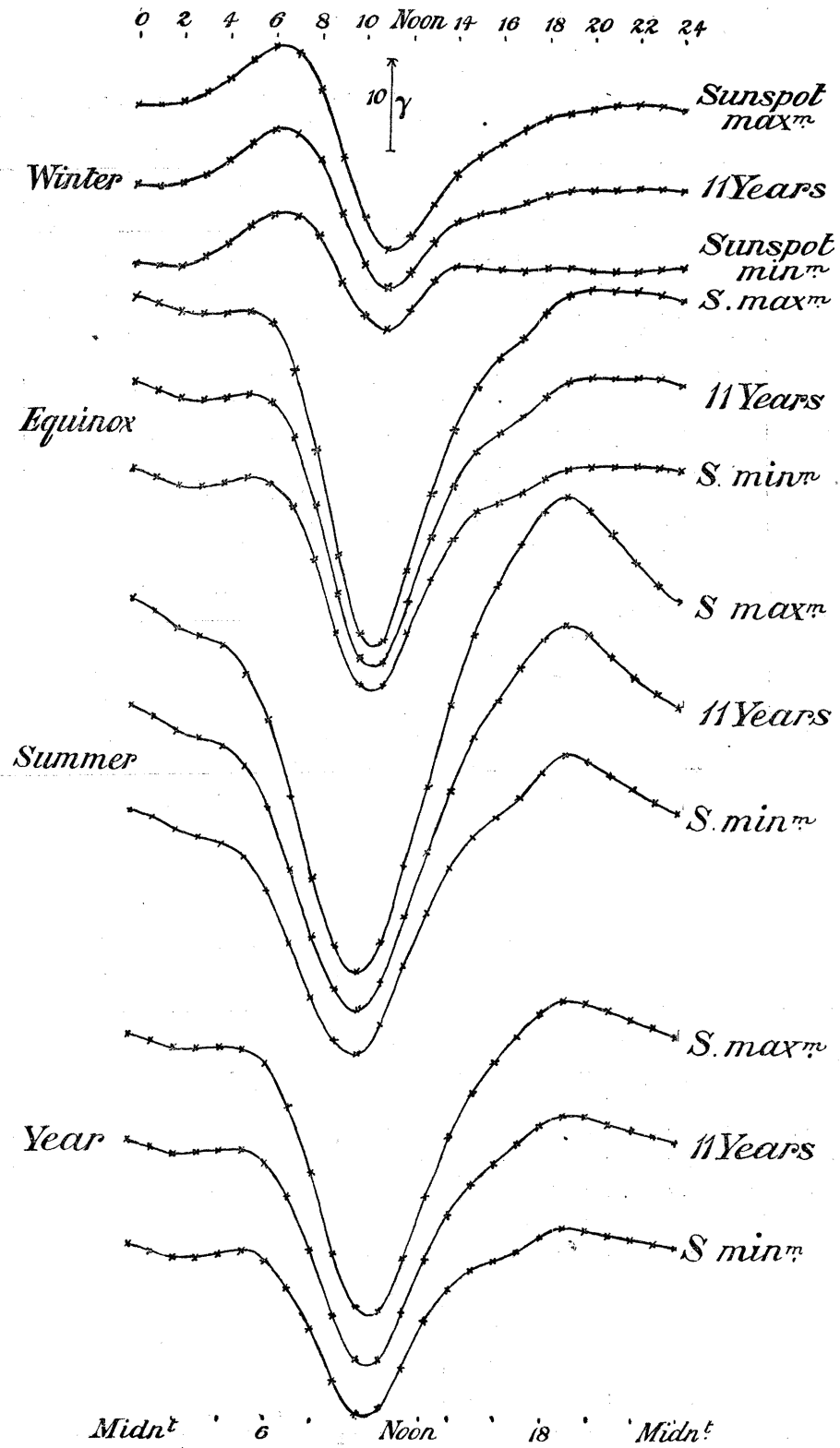
Fig. 2. Horizontal force.
