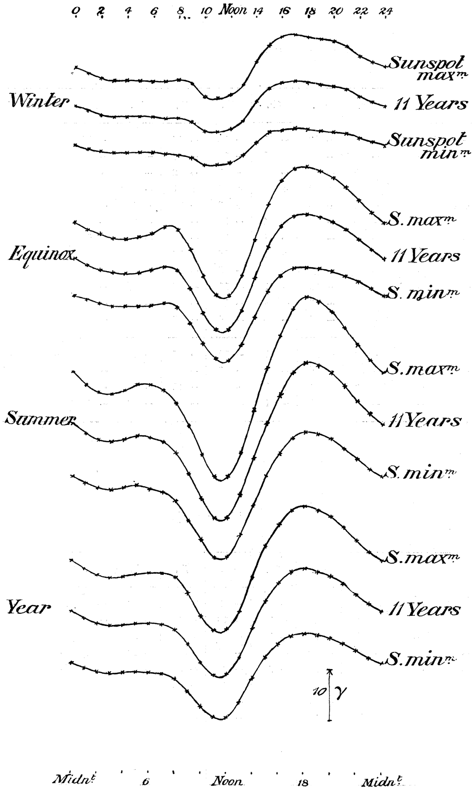
Fig. 4. Vertical force.
