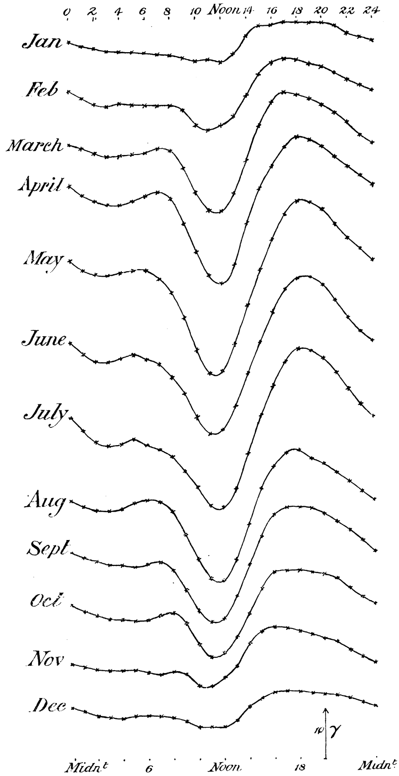
Fig. 3. Vertical force.
